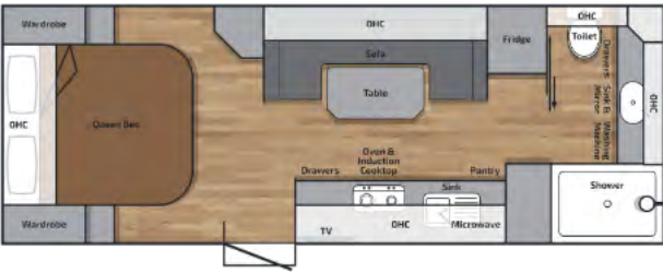
BR216CDQBSC External Body Length: 6590mm Overall Height: 3200mm Overall External Length: 9490mm Overall Width: 2500mm End Coupling to Outer Spare Tyre
