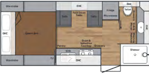
BR178RDQBDS External Body Length: 5420mm Overall Height: 3200mm Overall External Length: 8320mm Overall Width: 2500mm End Coupling to Outer Spare Tyre
