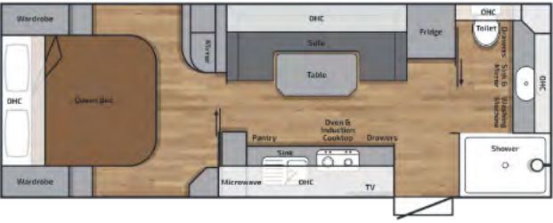
BR2111RDQBSC External Body Length: 6715mm Overall Height: 3200mm Overall External Length: 9625mm Overall Width: 2500mm End Coupling to Outer Spare Tyre
