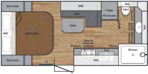
BR176CDQBLL External Body Length: 5365mm Overall Height: 3200mm Overall External Length: 8265mm Overall Width: 2500mm End Coupling to Outer Spare Tyre
