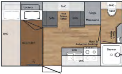
BR147CDQBEWDS External Body Length: 4480mm Overall Height: 3200mm Overall External Length: 7380mm Overall Width: 2500mm End Coupling to Outer Spare Tyre
