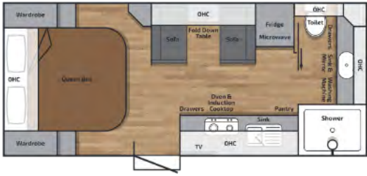
BR183CDQBDS External Body Length: 5595mm Overall Height: 3200mm Overall External Length: 8495mm Overall Width: 2500mm End Coupling to Outer Spare Tyre
