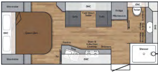
BR194RDQBDS External Body Length: 5925mm Overall Height: 3200mm Overall External Length: 8825mm Overall Width: 2500mm End Coupling to Outer Spare Tyre
