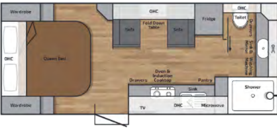
BR192CDQBDS External Body Length: 5875mm Overall Height: 3200mm Overall External Length: 8775mm Overall Width: 2500mm End Coupling to Outer Spare Tyre
