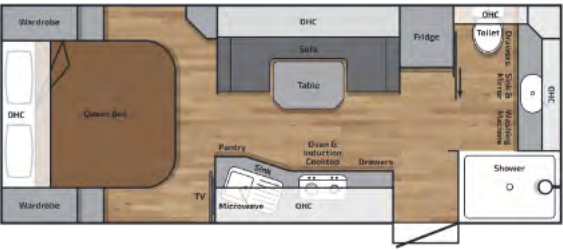
BR1911RDQBSC External Body Length: 6105mm Overall Height: 3200mm Overall External Length: 9005mm Overall Width: 2500mm End Coupling to Outer Spare Tyre
