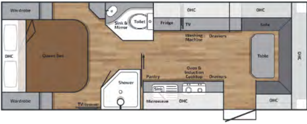
BR2111RDQBRC External Body Length: 6715mm Overall Height: 3200mm Overall External Length: 9625mm Overall Width: 2500mm End Coupling to Outer Spare Tyre
