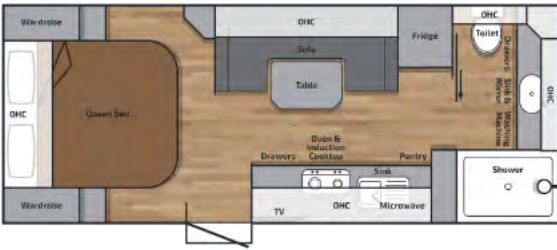
BR199CDQBSC External Body Length: 6055mm Overall Height: 3200mm Overall External Length: 8955mm Overall Width: 2500mm End Coupling to Outer Spare Tyre
