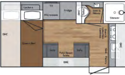
BR149RDQBEWDS External Body Length: 4530mm Overall Height: 3200mm Overall External Length: 7430mm Overall Width: 2500mm End Coupling to Outer Spare Tyre
