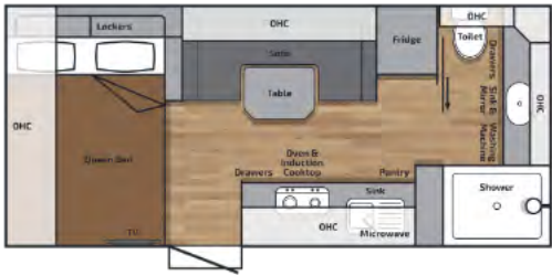
BR176CDQBEWSC External Body Length: 5365mm Overall Height: 3200mm Overall External Length: 8265mm Overall Width: 2500mm End Coupling to Outer Spare Tyre
