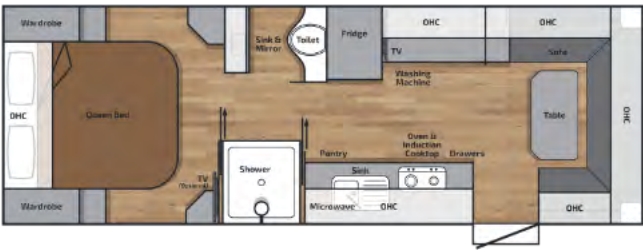
BR228RDQBRC External Body Length: 6945mm Overall Height: 3200mm Overall External Length: 9845mm Overall Width: 2500mm End Coupling to Outer Spare Tyre
