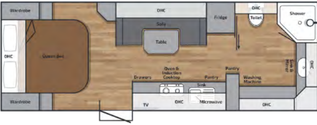
BR226CDQBSC External Body Length: 6895mm Overall Height: 3200mm Overall External Length: 9805mm Overall Width: 2500mm End Coupling to Outer Spare Tyre
